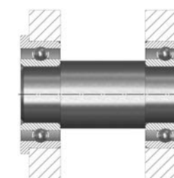
Assembly in narrow housings
