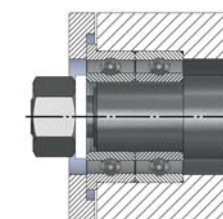
Application of a Duplex bearing
